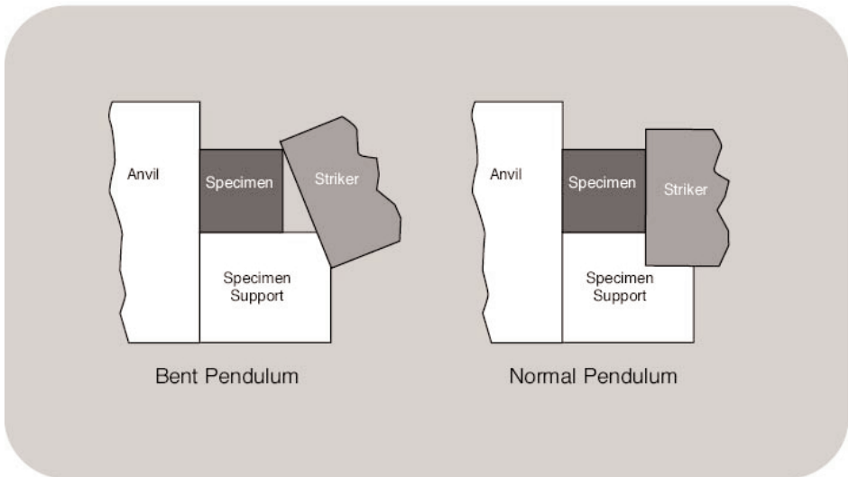
Figure 8. Bent Pendulum.
