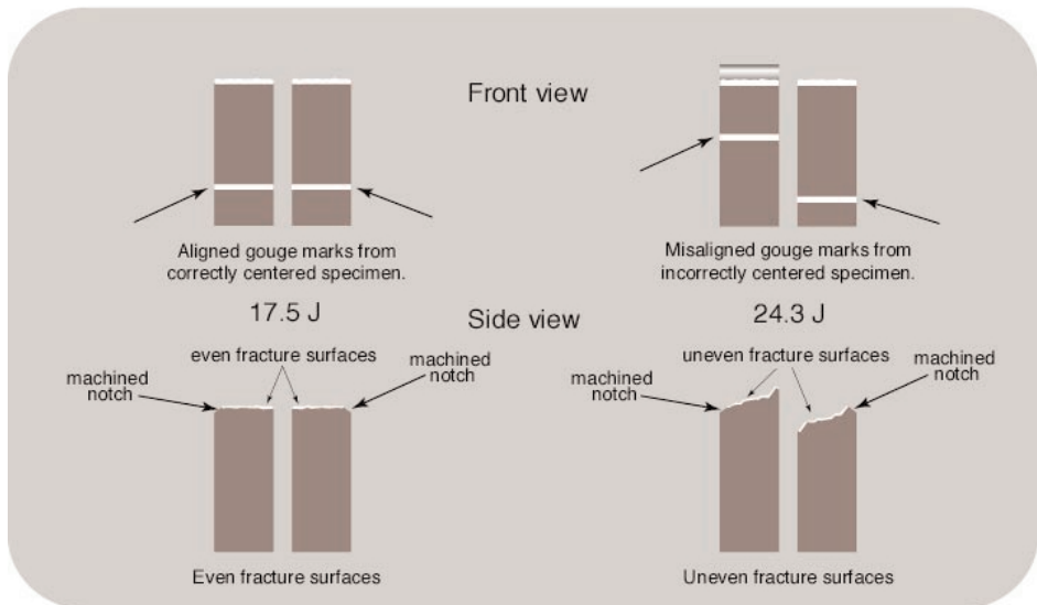
Figure 2. Off-Center Specimen.
